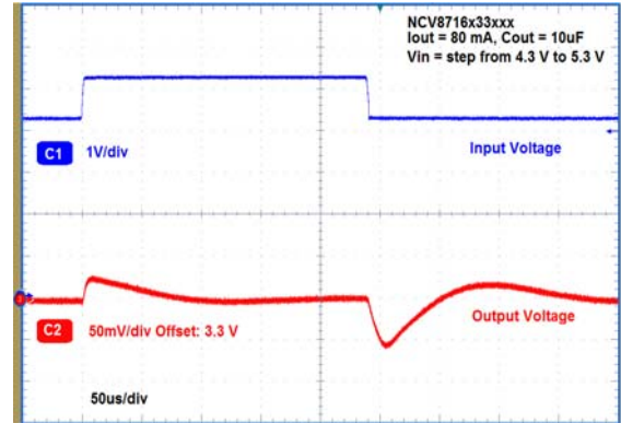
Figure 36. Line Transient Response
