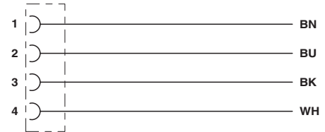
Contact assignment of the DEUTSCH DT06-4S
