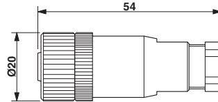
Dimensioned drawing
