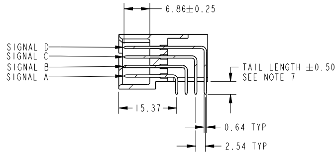
SECTION C-C SCALE 1:1 FOR SIGNAL SOLDER TO BOARD ONLY
