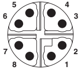
Pin assignment M12 plug, 8-pos., view plug side
