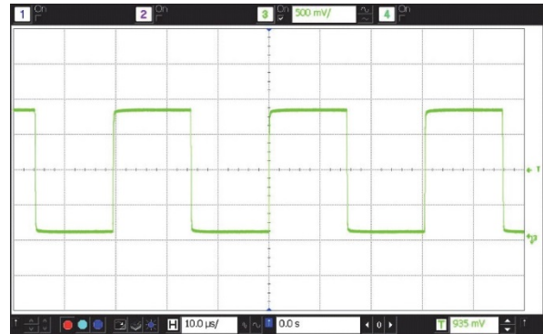
Figure 3. LVCMOS Waveform (V DD = 1.8V) into 15 pF Load
