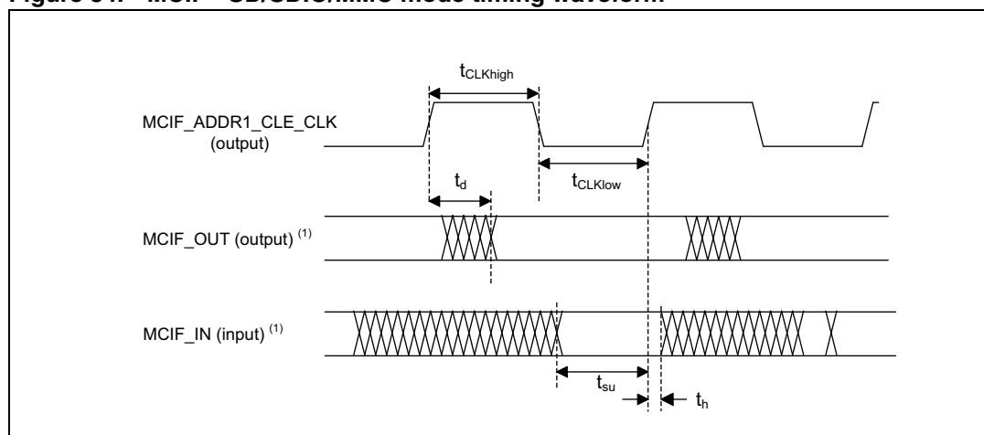
Figure 34. MCIF - SD/SDIO/MMC mode timing waveform
