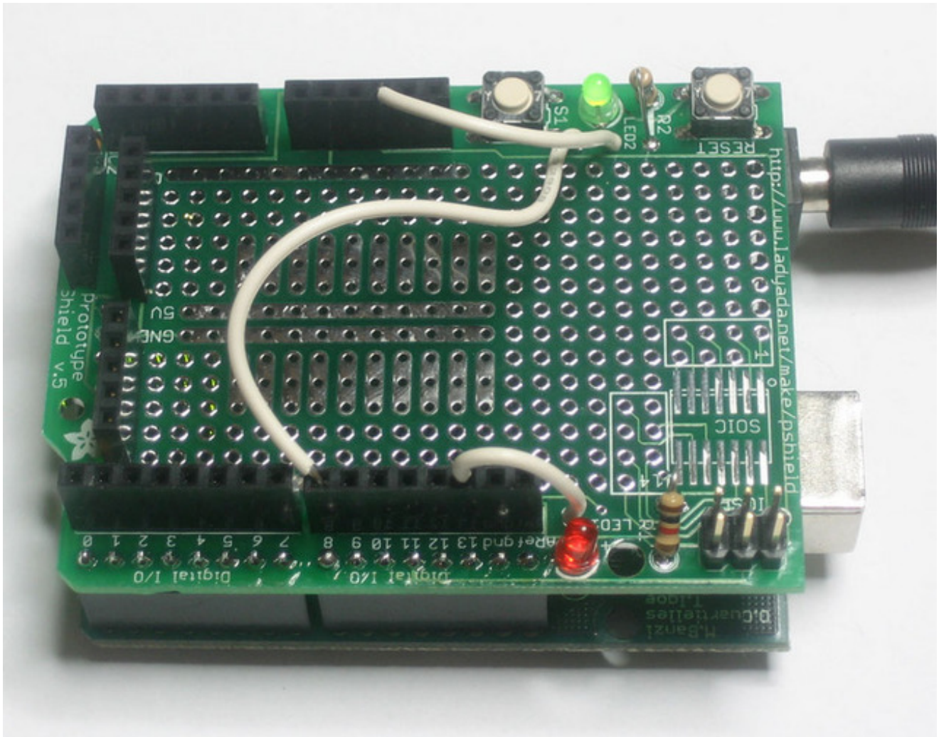
2 LEDs and one button are available for general purpose use!
